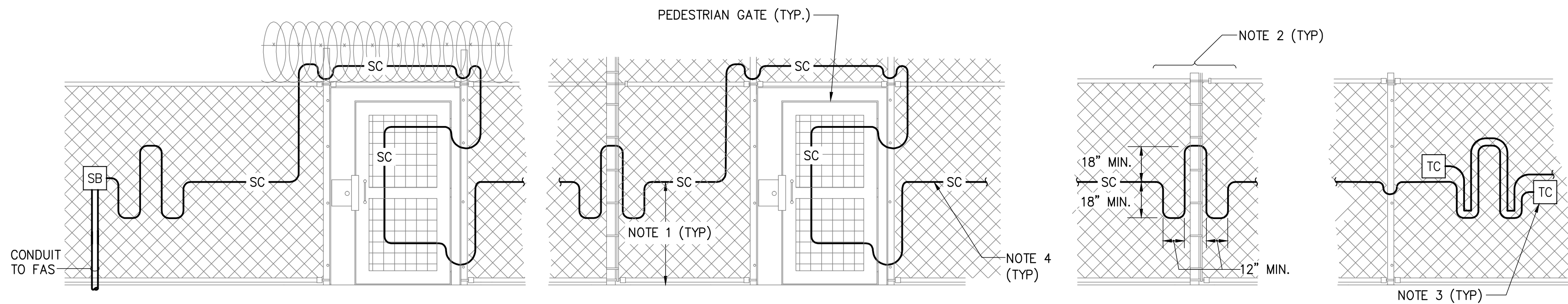
ELEVATION – SENSOR CABLE INSTALLATION ON FENCE (TYPICAL)
