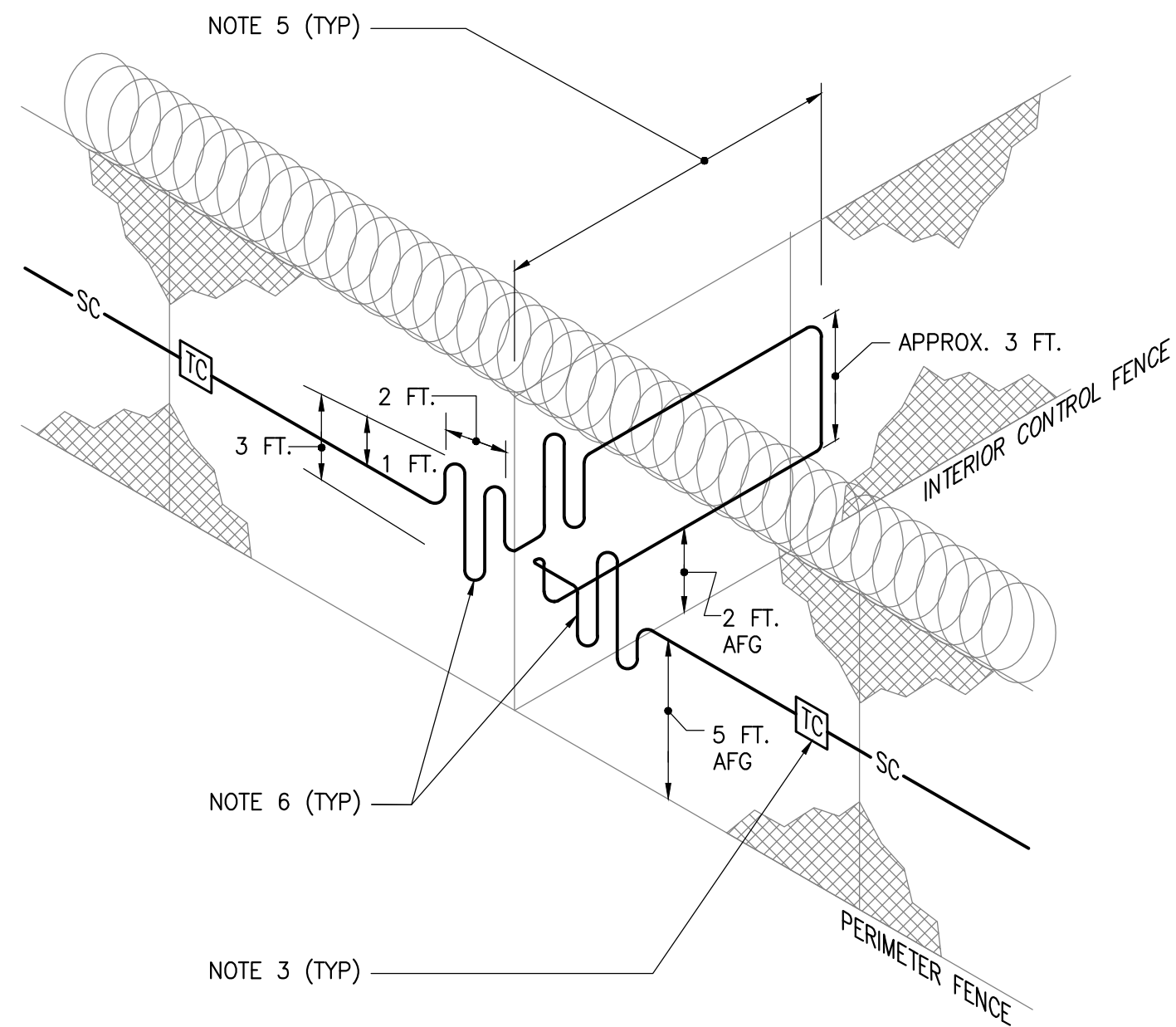
ISOMETRIC VIEW OF TYPICAL INSTALLATION OF SENSOR CABLE WHERE INTERIOR CONTROL FENCE INTERSECTS PERIMETER FENCE
