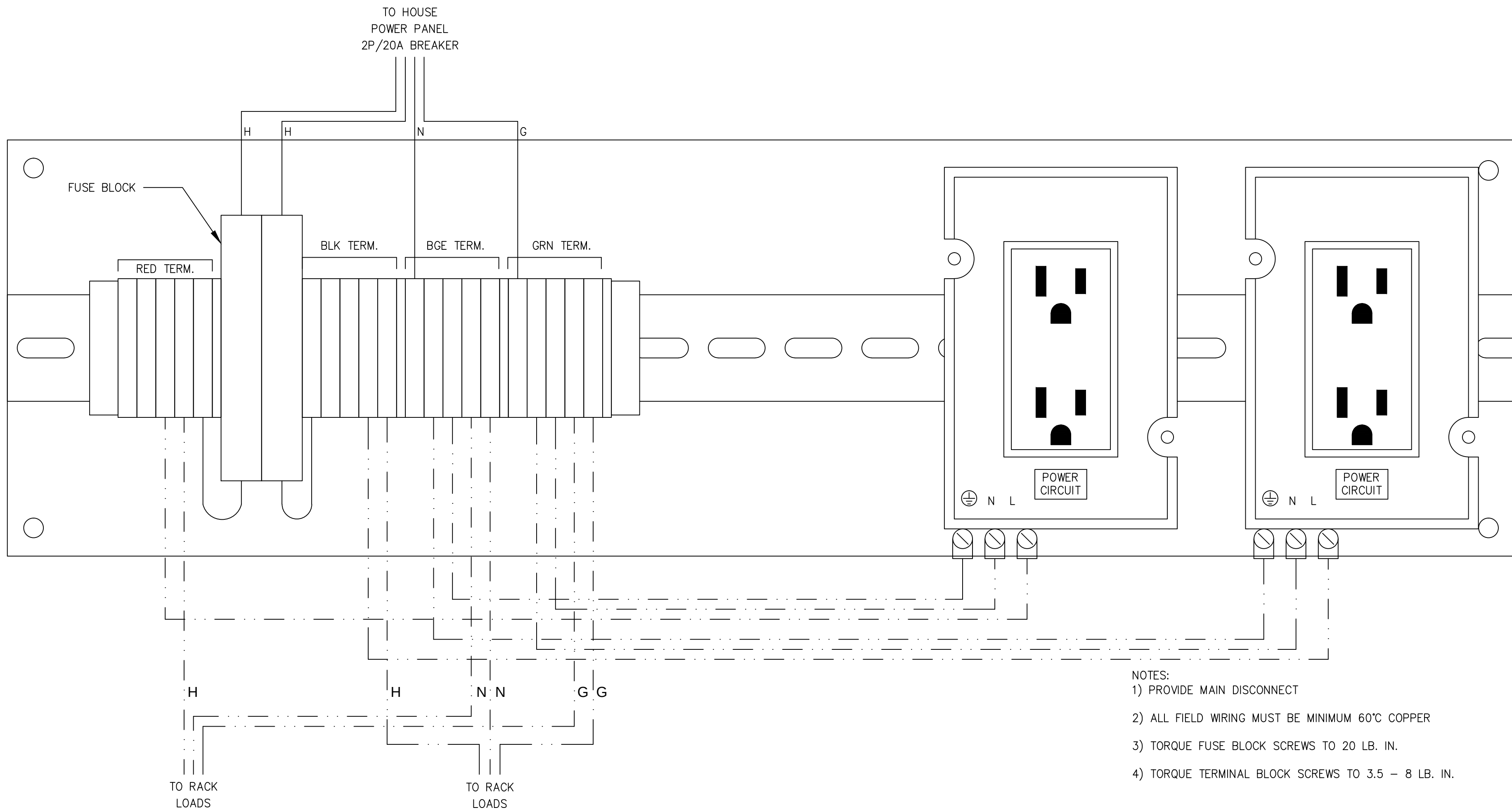
1 POWER DISTRIBUTION WIRING DETAIL - NOT TO SCALE
