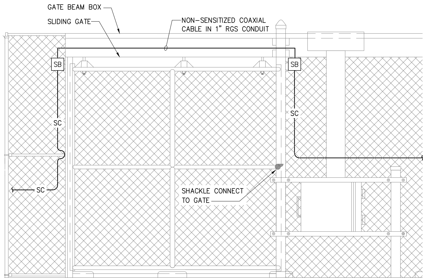
ELEVATION – SENSOR CABLE INSTALLATION ON SLIDING GATE
