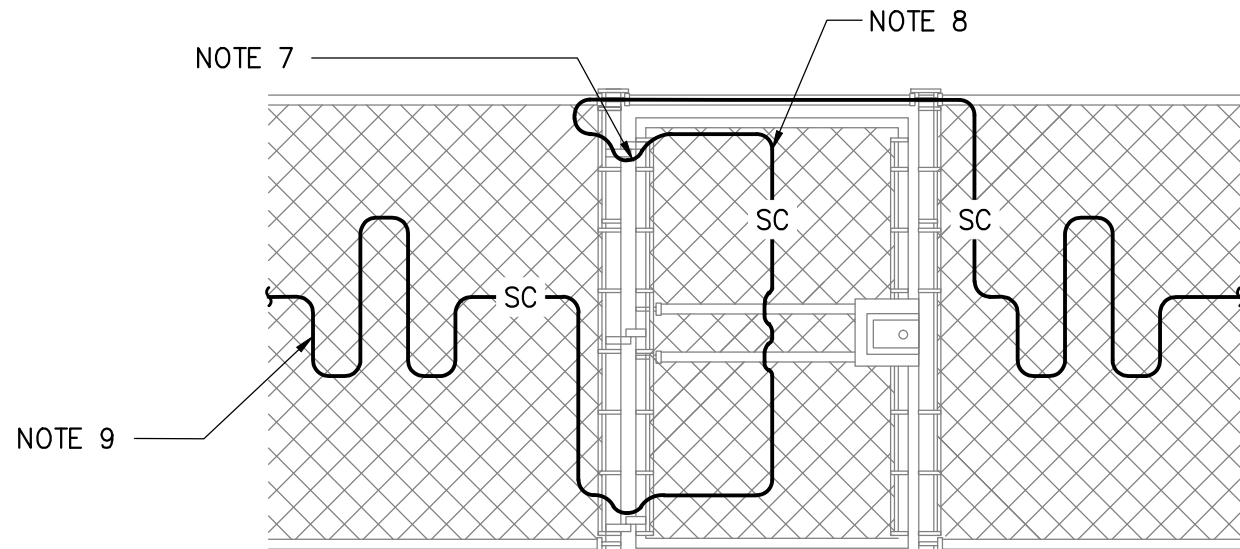
ELEVATION – SENSOR CABLE INSTALLATION ON MAINTENANCE GATE
